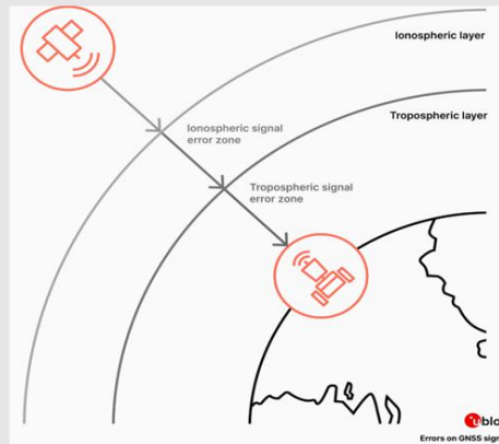
How RTK Differs from Traditional GNSS Positioning
